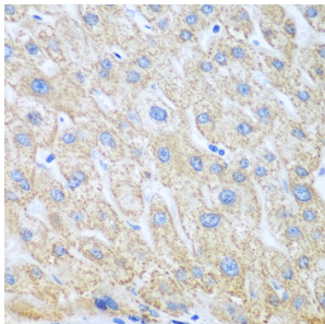
Immunohistochemistry analysis of paraffin-embedded Human liver cancer using COX1/PTGS1 Rabbit pAb (A7341) at dilution of 1:100 (40x lens). Microwave antigen retrieval performed with 0.01M PBS Buffer (pH 7.2) prior to IHC staining.
