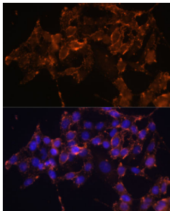
Immunofluorescence analysis of HeLa cells using COX1/PTGS1 Rabbit pAb (A7341) at dilution of 1:100 (40x lens). Secondary antibody: Cy3-conjugated Goat anti-Rabbit IgG (H+L) (AS007) at 1:500 dilution. Blue: DAPI for nuclear staining.
