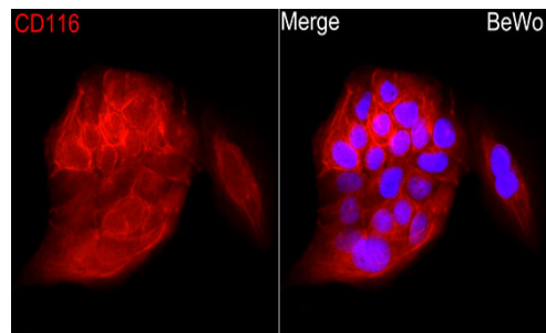
Immunofluorescence analysis of BeWo cells using CSF2RA Rabbit pAb (A3167) at dilution of 1:200 (40x lens). Secondary antibody: Cy3-conjugated Goat anti-Rabbit IgG (H+L) (AS007) at 1:500 dilution. Blue: DAPI for nuclear staining.
