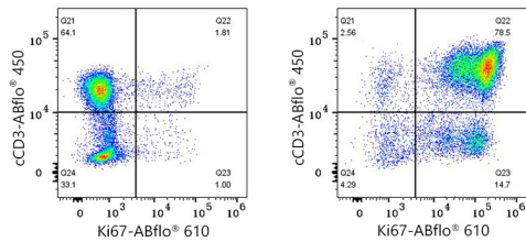
Flow cytometry: 1X10^6 Human PBMC (untreated,left) and Human PBMC (treated with 5 µg/mL PHA for 72 hours,right) were intracellularly-stained with ABflo® 450 Rabbit anti-Human cCD3 mAb (A27836,5 µl/Test) and ABflo® 610 Rabbit anti-Human/Monkey Ki67 mAb (A26736,5 µl/Test). Cells in the lymphocyte gate were used for analysis.
