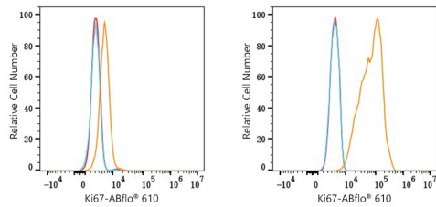
Flow cytometry: 1X10^6 knockout (KO) HeLa cells (negative control,left) and HeLa cells (right) were intracellularly-stained with ABflo® 610 Rabbit anti-Human/Monkey Ki67 mAb (A26736,5 µl/Test,orange line) or ABflo® 610 Rabbit IgG isotype control (A25826,5 µl/Test,blue line). Non-fluorescently stained cells were used as blank control (red line).
