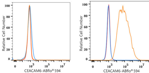
Flow cytometry: 1X10^6 HeLa cells (negative control,left) and BxPC-3 cells (right) were surface-stained with ABflo® 594 Rabbit anti-Human CEACAM6 mAb (A24188,5 µl/Test,orange line) or ABflo® 594 Rabbit IgG isotype control (A23821,5 µl/Test,blue line). Non-fluorescently stained cells were used as blank control (red line).
