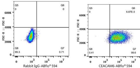
Flow cytometry: 1X10^6 BxPC-3 cells were surface-stained with ABflo® 594 Rabbit IgG isotype control (A23821,5 µl/Test,left) or ABflo® 594 Rabbit anti-Human CEACAM6 mAb (A24188,5 µl/Test,right).
