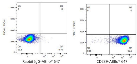
Flow cytometry:1X10 6 SK-BR-3 cells were surface-stained with ABflo ® 647 Rabbit IgG isotype control (A22070,5 µl/Test,left) or ABflo ® 647 Rabbit anti-Human CD239/BCAM mAb(A23745,5 µl/Test,right).
