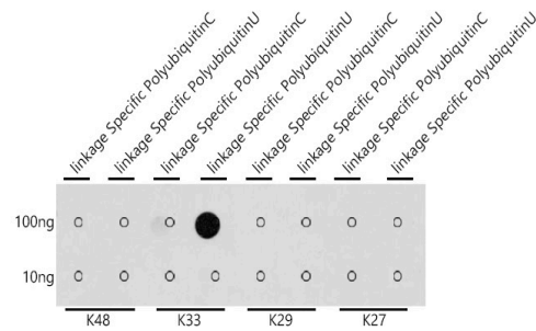
Dot-blot analysis of all sorts of peptides using K33-linkage Specific Polyubiquitin antibody (A18199) at 1:1000 dilution.
